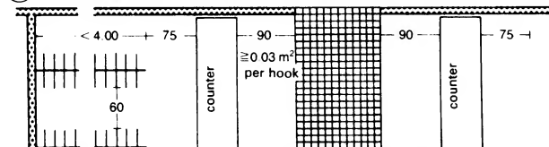
⑦ Supervised cloakroom, with racks of coat-hangers
